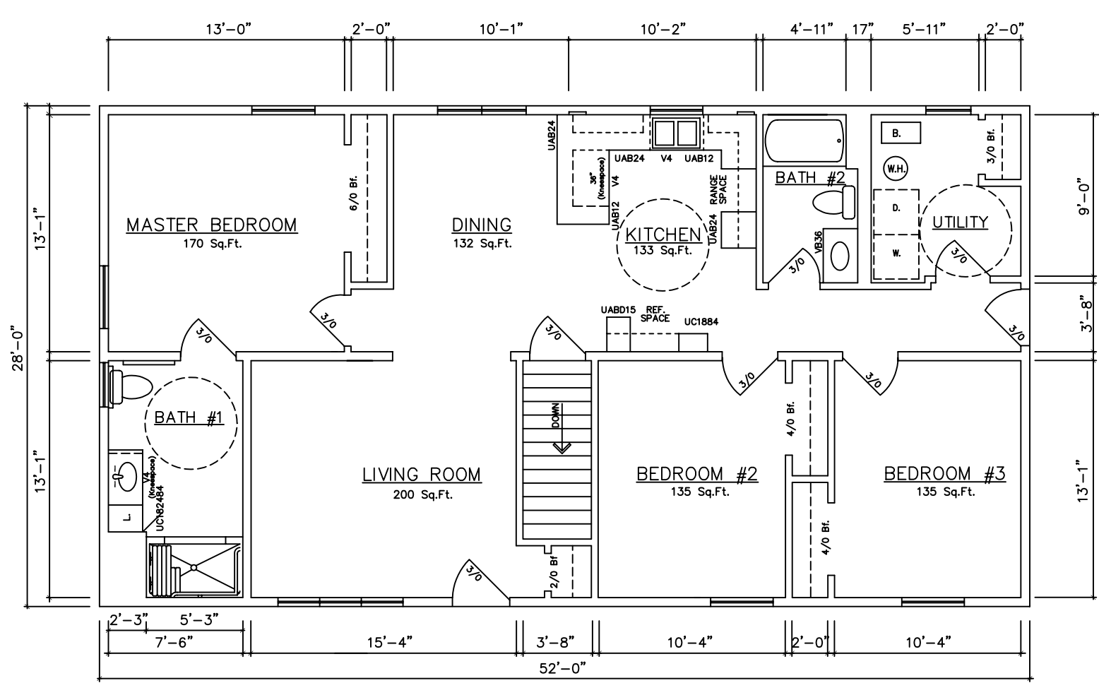
GROUND FLOOR PLAN (BASEMENT)
