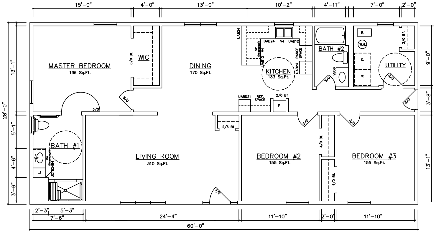
GROUND FLOOR PLAN (CRAWL)
