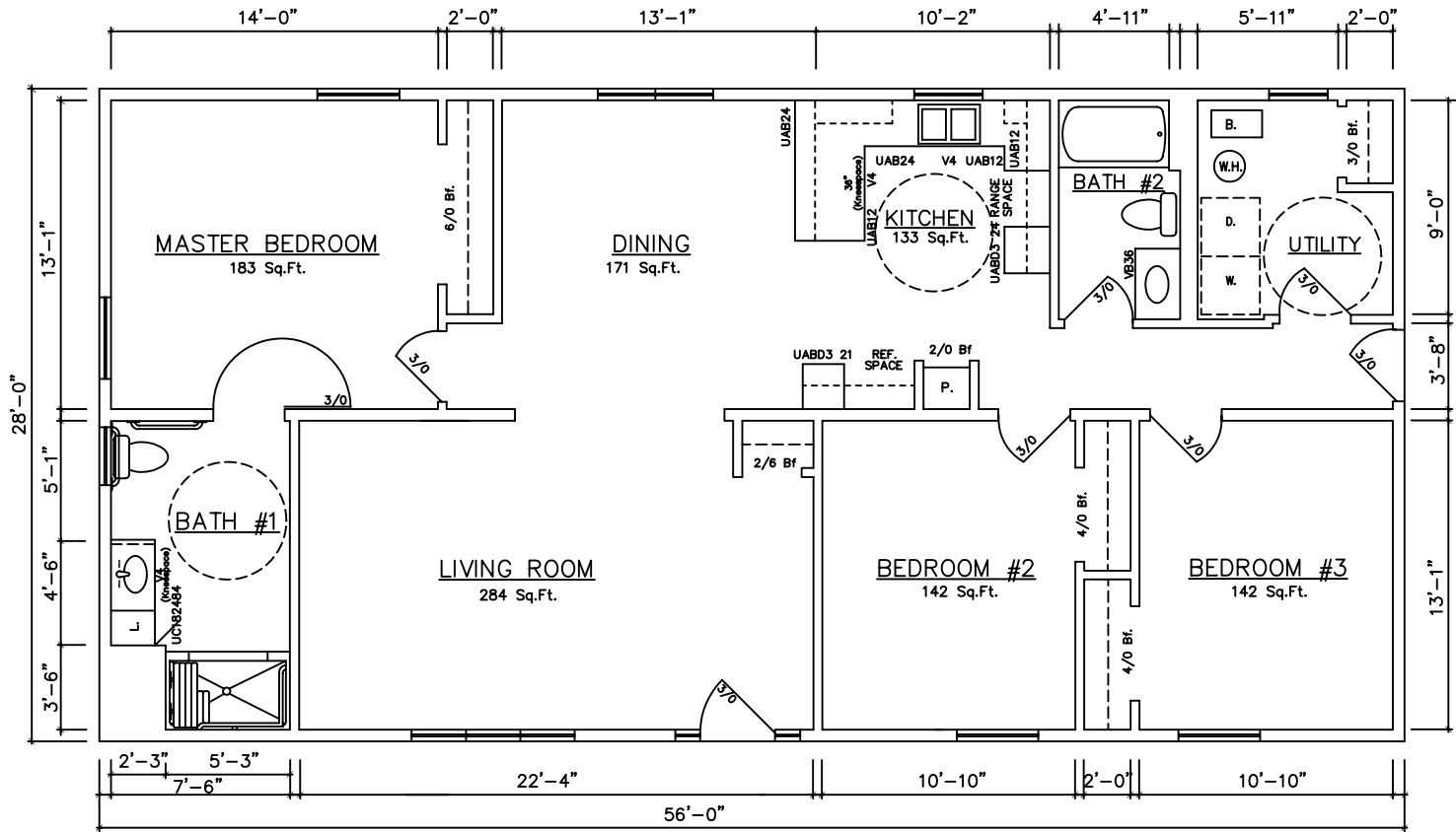
GROUND FLOOR PLAN (BASEMENT)
